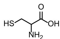
cysteine
